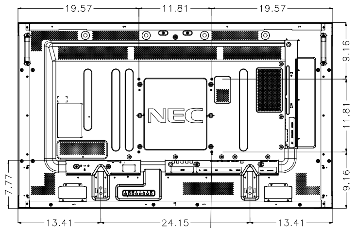
300mm MOUNTING HOLE PATTERN FOR MOUNT UNIT (M6 Depth 12mm)
